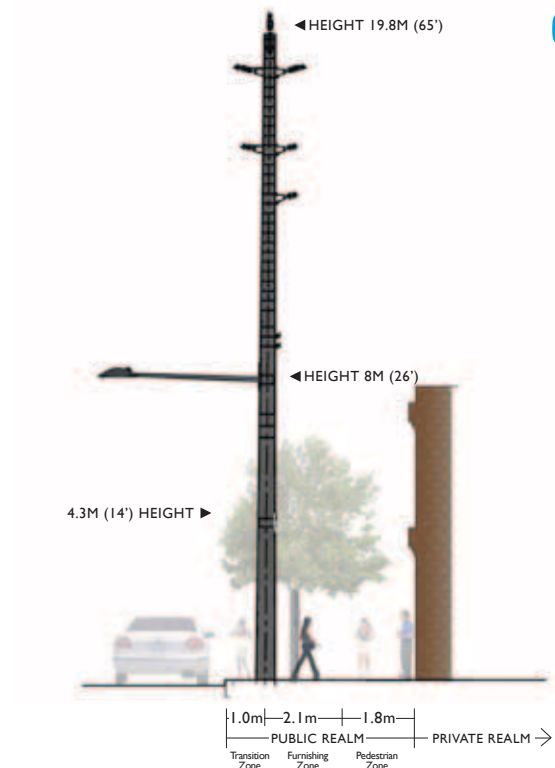
Pedestrian / vehicle cross section
